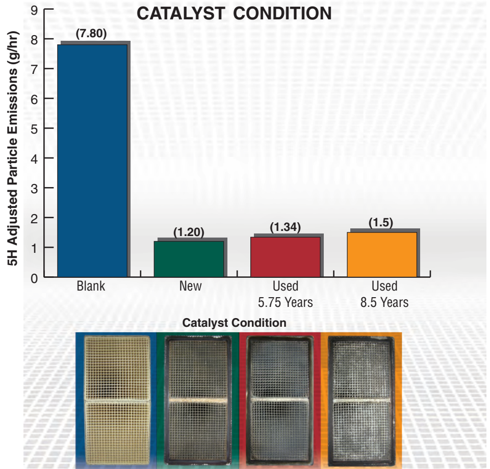
Particulate emissions are nearly as low in older catalysts as new ones when used in a well-designed stove. Two to three cords per year were burned in the used catalytic stoves.
