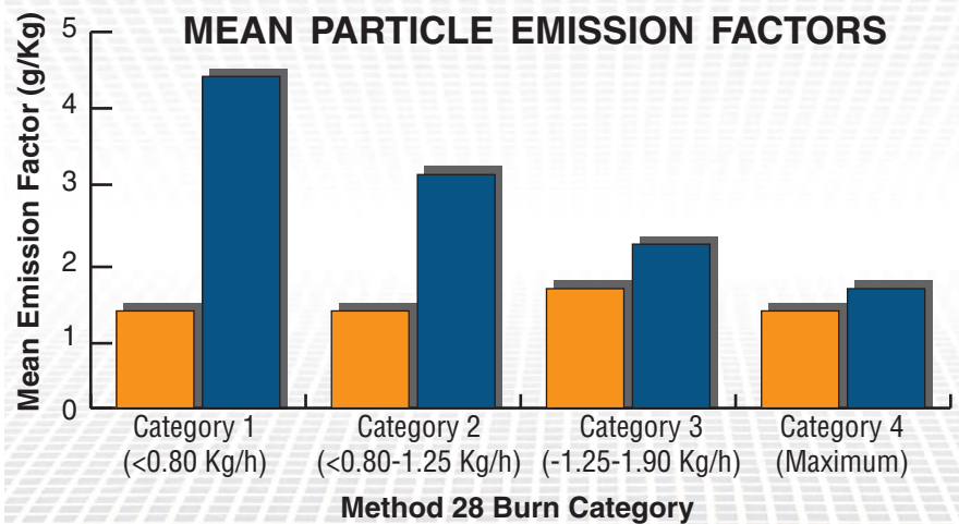
Mean particulate emission factors for certified catalytic heaters are less than for non-catalytic heaters at all burn rates. (Data after Ferguson, Andors & Company 2010 report to HPBA.) Most dramatic is the difference at low-burn rates which would be more prevalent in milder climates and at the margins (Spring and Autumn) of the heating season.
