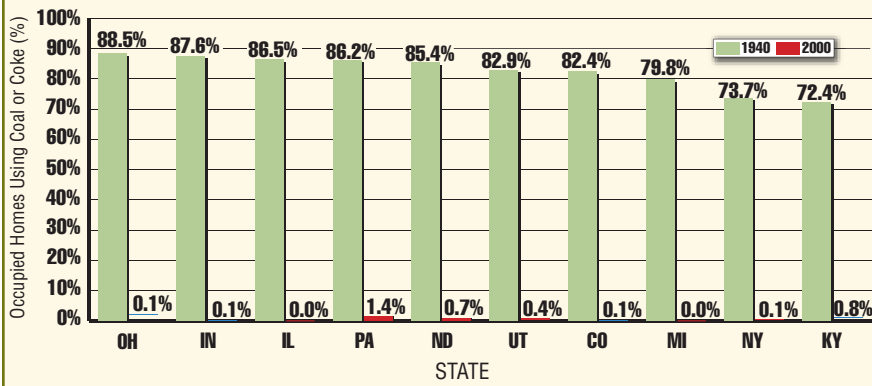
The percentage of households using coal as a heating fuel in key coal using states in 1940 and 2000 (U.S. Census Bureau).
