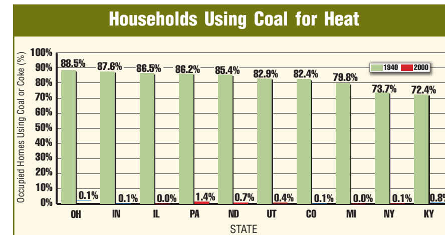
The percentage of households using coal as a heating fuel in key coal using states in 1940 and 2000 (U.S. Census Bureau).
